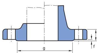
RAISED FACE (LARGE)
