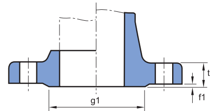
RAISED FACE (SMALL)
